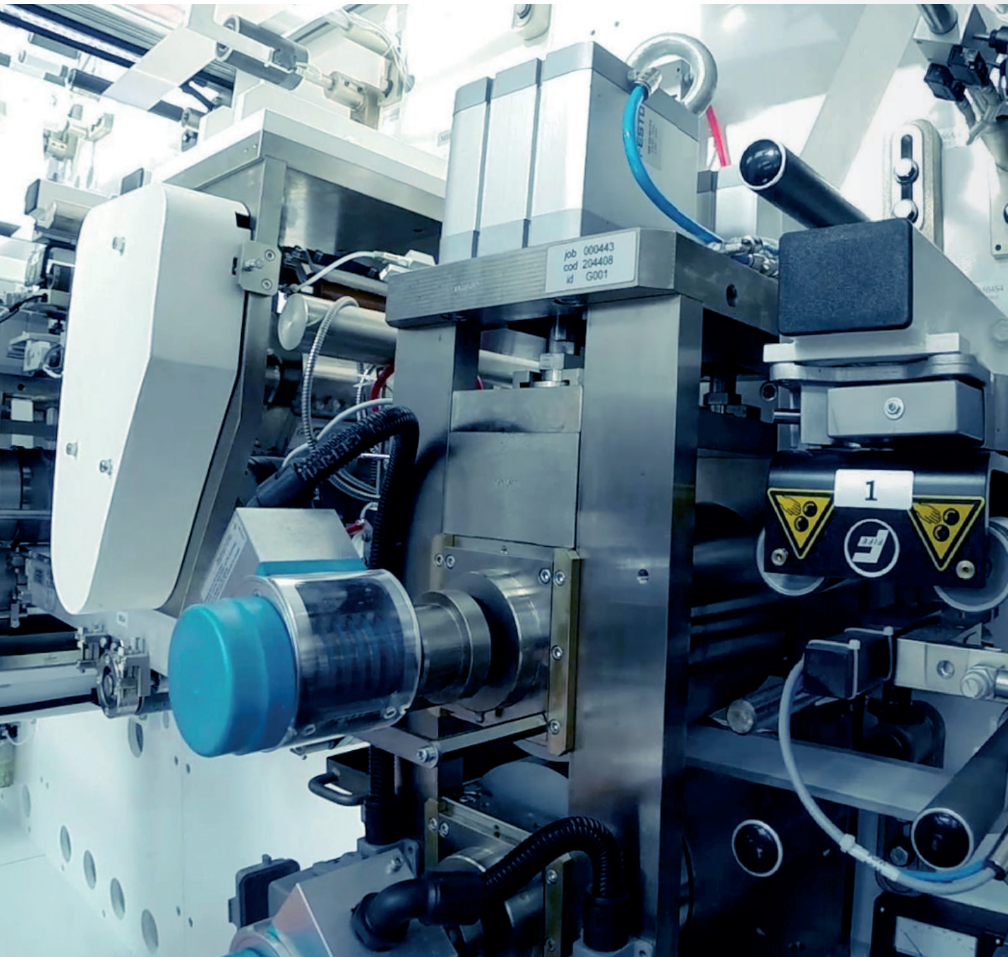
Dimpling unit
