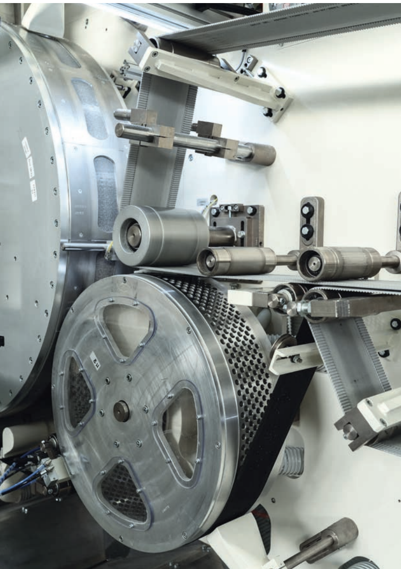
Offline unwinders
